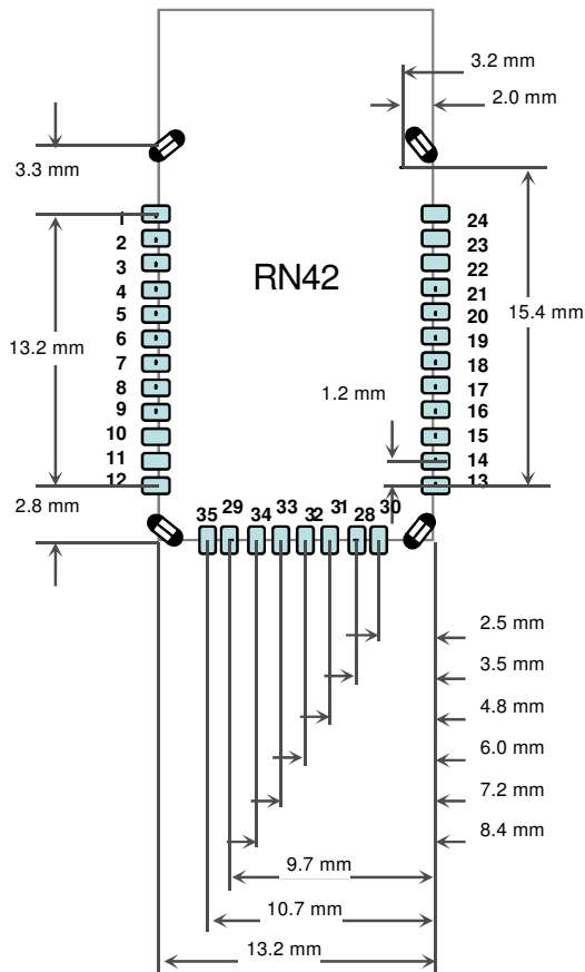
PCB LAYOUT PAD SIZE = 0.8 X 1.30 mm (TOP VIEW)
